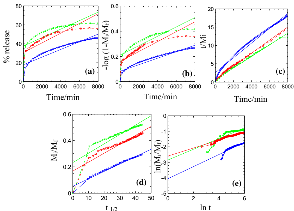
Fig. 14 Fitting data of the FZ release data into 0.3 (blue), 0.5 (red) and 1.0 (green) M concentration of chloride solution to the a zeroth order model, b first order model, c pseudo- second order model, d parabolic diffusion model and e fickian diffusion model (Color figure online)
