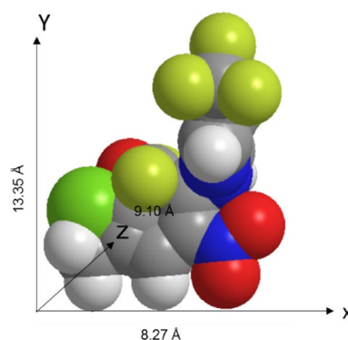
Fig. 4 3-D molecular structure of the FZ
