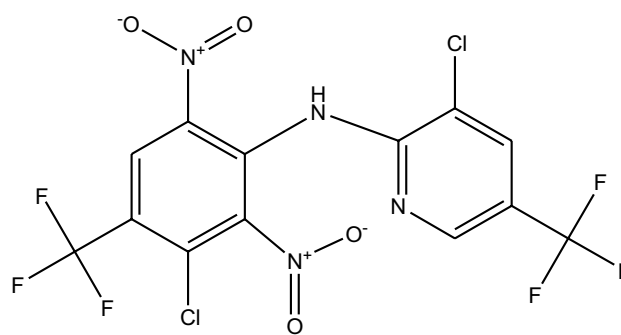
Fig. 1 The chemical structure of fluazinam
