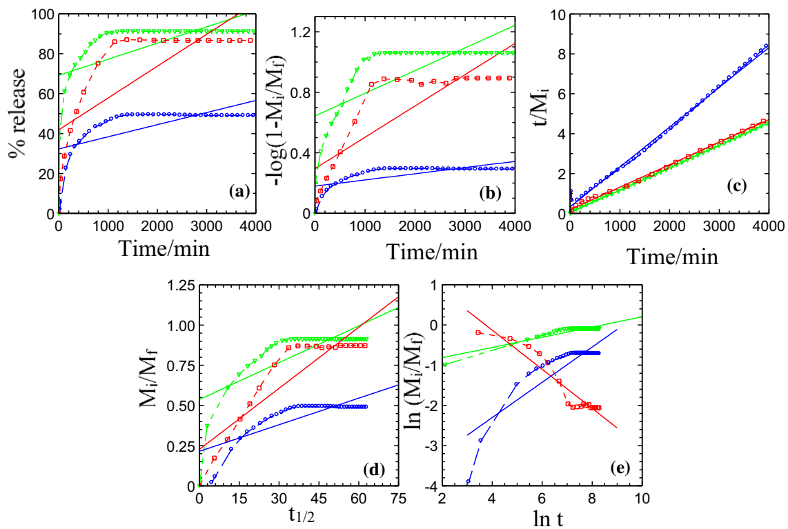
Fig. 12 Fitting data of the FZ release data into 0.3 (blue), 0.5 (red) and 1.0 (green) M concentration of phosphate solution to the a zeroth order model, b first order model, c pseudo- second order model, d parabolic diffusion model and e fickian diffusion model (Color figure online)
