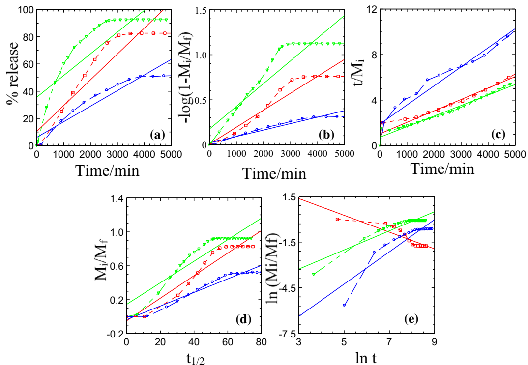
Fig. 13 Fitting data of the FZ release data into 0.3 (blue), 0.5 (red) and 1.0 (green) M concentration of carbonate at the a zeroth order model, b first order model, c pseudo- second order model, d parabolic diffusion model and e fickian diffusion model (Color figure online)
