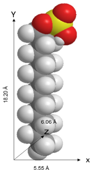
Fig. 3 3-D molecular structure of the SDS
