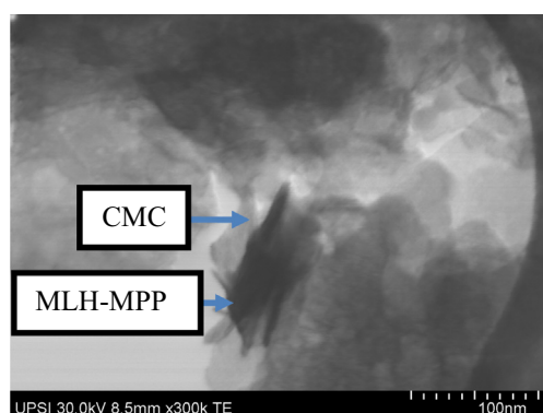
Fig. 5 TEM micrograph of MLH-MPP/CMC nanocomposite at 300 k magnification.
