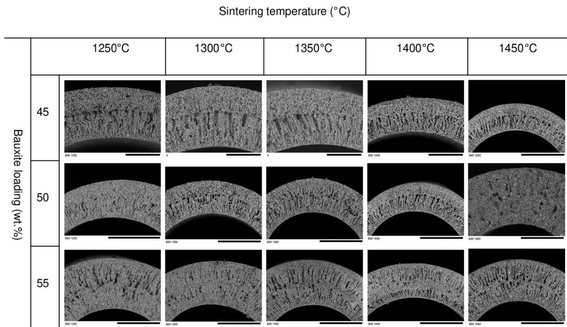
Fig. 5. Microscopic images of BHF membrane fabricated with various bauxite loadings and sintering temperatures. Scale bars: top row (1–4) – 100 \mu\text{m} ; top row (5) and middle and bottom rows – 300 \mu\text{m}
